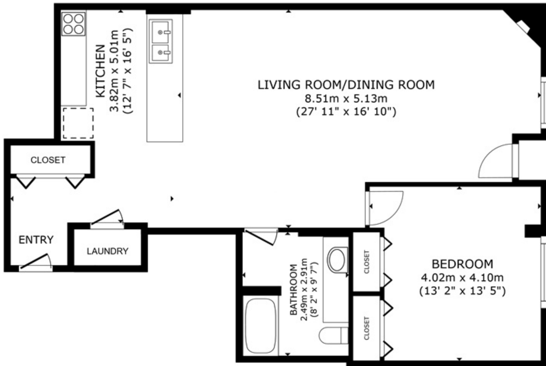
FLOOR PLAN
